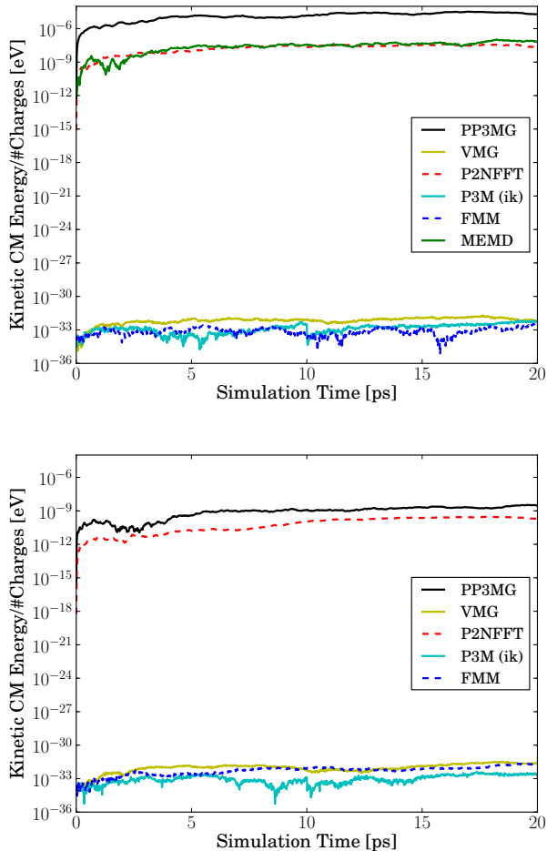
Figure 6. Kinetic energy per particle of the center-of-mass motion of the system according to different methods and accuracies: \epsilon_{\text{pot}} = 10^{-3} (top), \epsilon_{\text{pot}} = 10^{-5} (bottom). Note that the P 3 M method used here differs from the P 3 M method in the other plots as described in the text. With MEMD, only an accuracy of \epsilon_{\text{pot}} = 10^{-3} could be reached.
