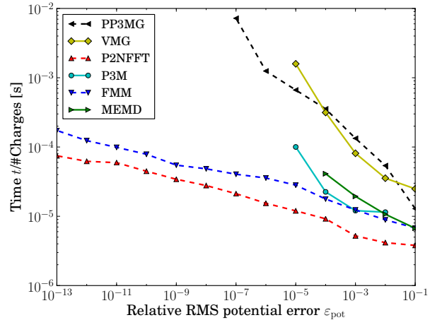
Figure 8. Required wall clock time per particle for 102 900 charges versus the relative RMS potential error \varepsilon_{\text{pot}} on 1 core of JUROPA.
